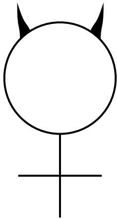
Mercury
